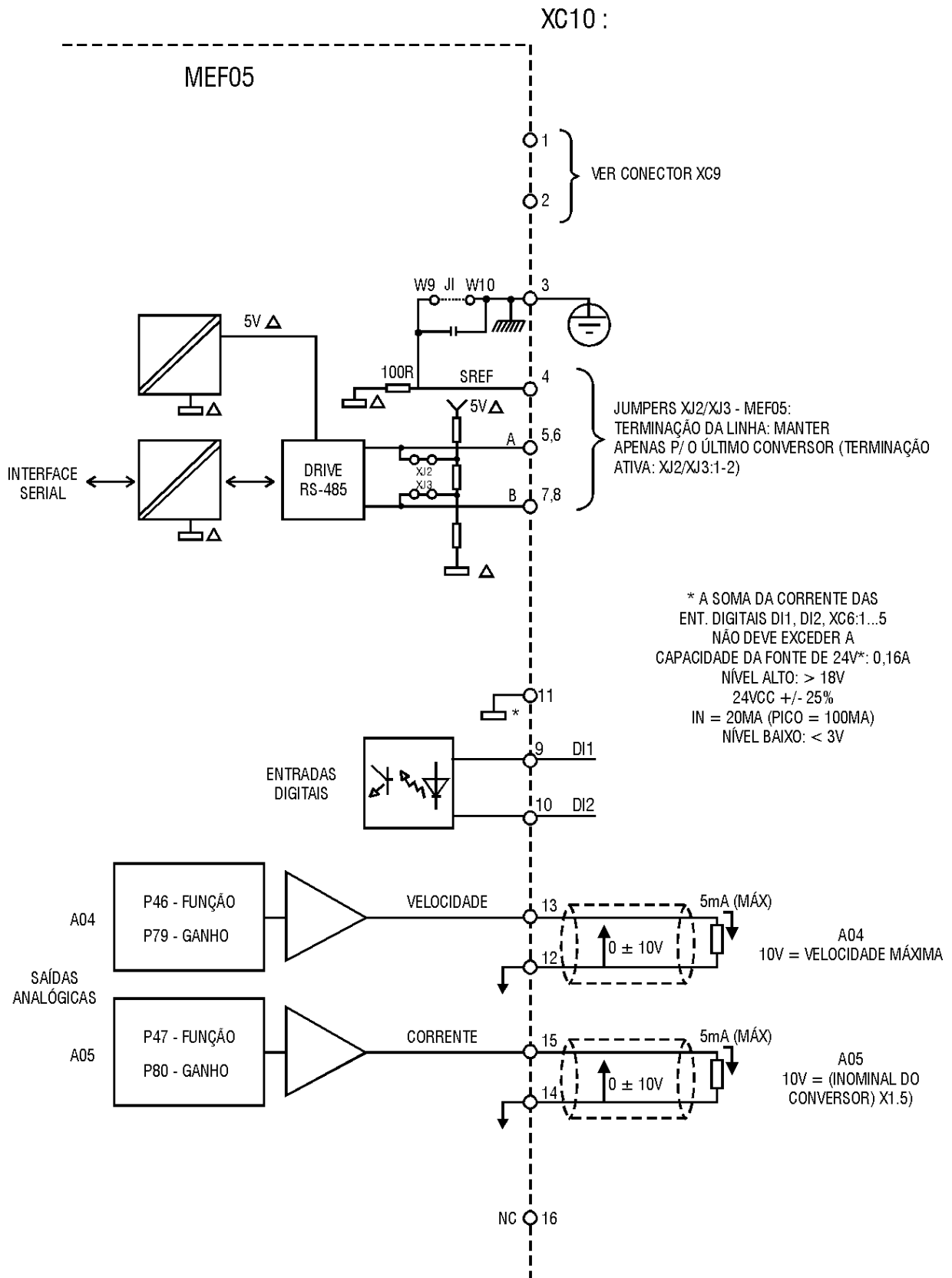
Figura 1.7.2 - Conector XC10 - MEF-05
